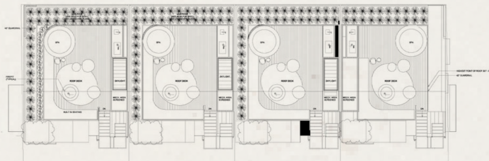
ROOF PLAN
